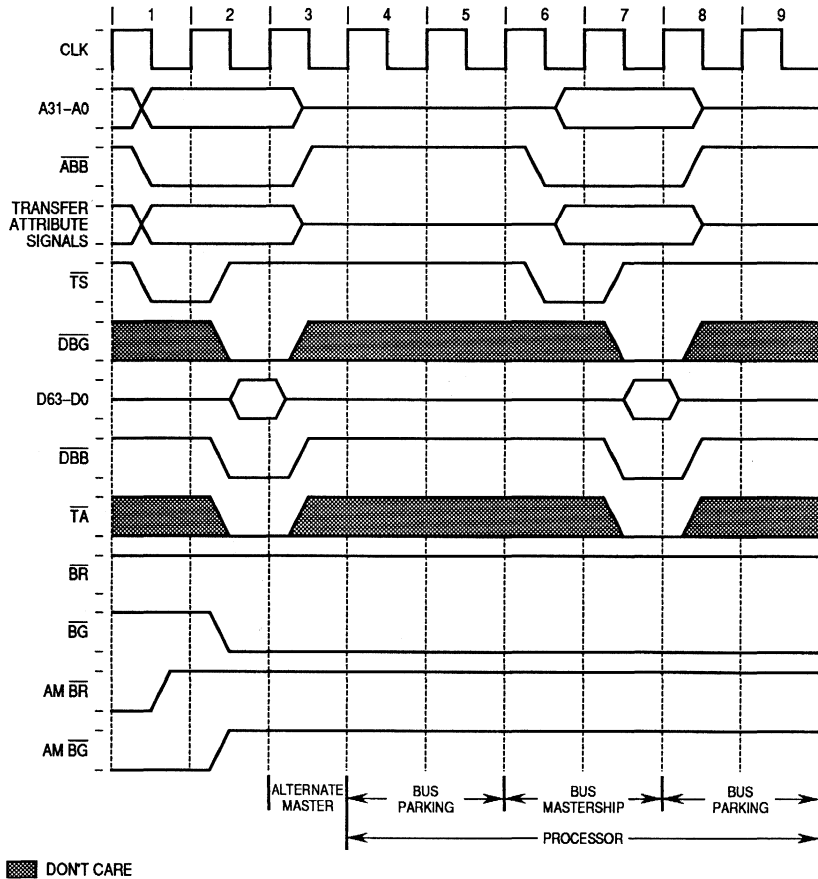
Figure 11-16. Bus Parking
