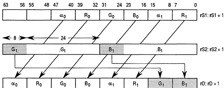
Figure 5-5. ppack.16 rD,rS1,rS2
