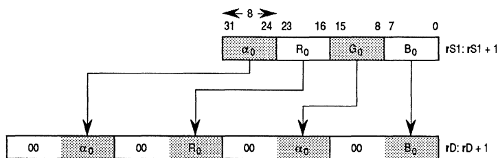
Figure 5-6. punpk.b rD,rS1
