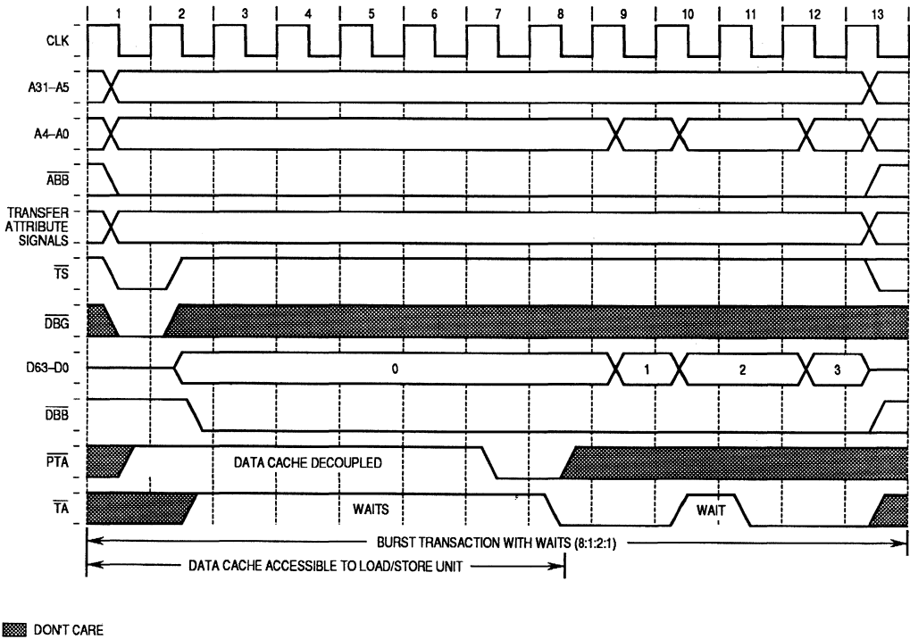
Figure 11-37. Normal Termination of a Burst Transaction with \overline{PTA} and \overline{TA}
