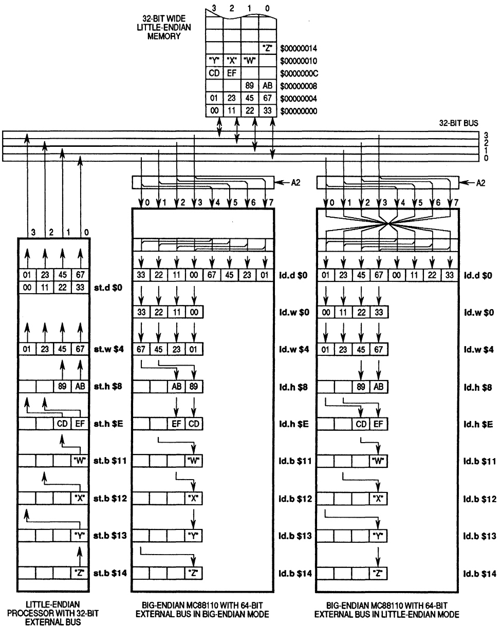
Figure 2-12. Example Byte-Ordering Environment Using Little-Endian Memory and 32-Bit Bus
