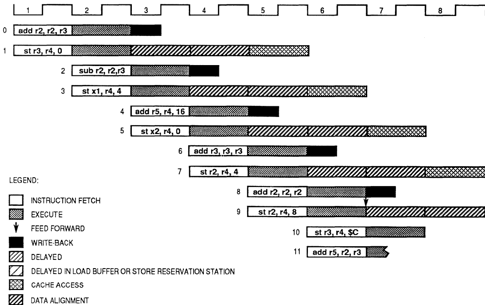
Figure 9-25. Store Timing
