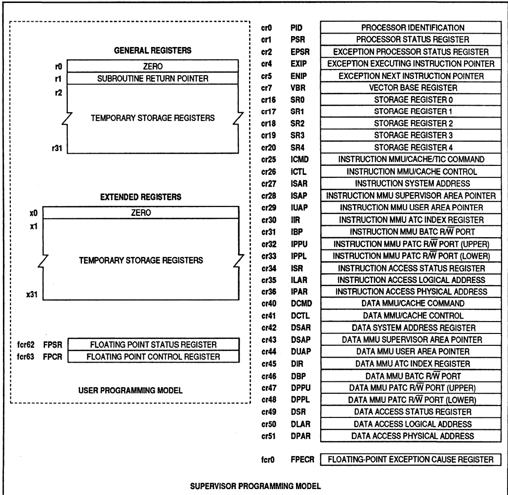
Figure 2-1. Programming Model
