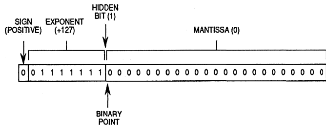
Figure 4-2. Single-Precision Floating-Point Representation of 1.0
