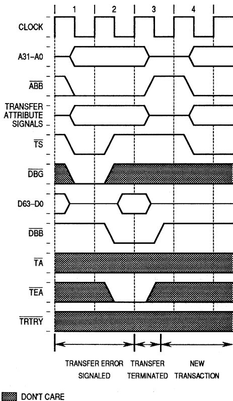
Figure 11-41. Transfer Error Termination
