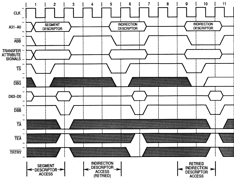
Figure 11-54. Hardware Table Search with \overline{\text{TRTRY}} (Sheet 1 of 2)
