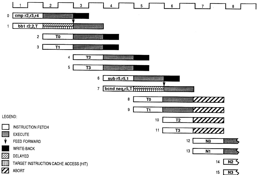
Figure 9-42. Predicted Branch Taken Timing
