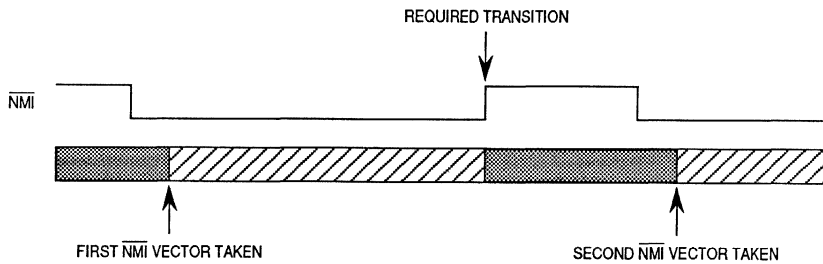
Figure 7-9. \overline{\text{NMI}} Signal Timing
