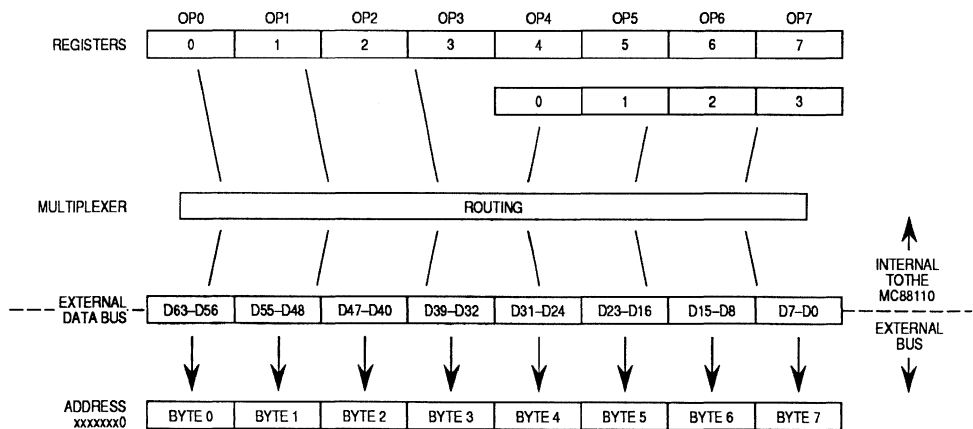
Figure 11-21. Data Multiplexing
