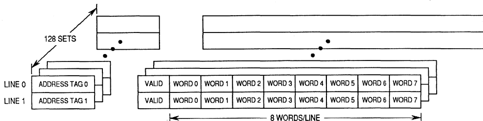
Figure 1-4. Instruction Cache Organization
