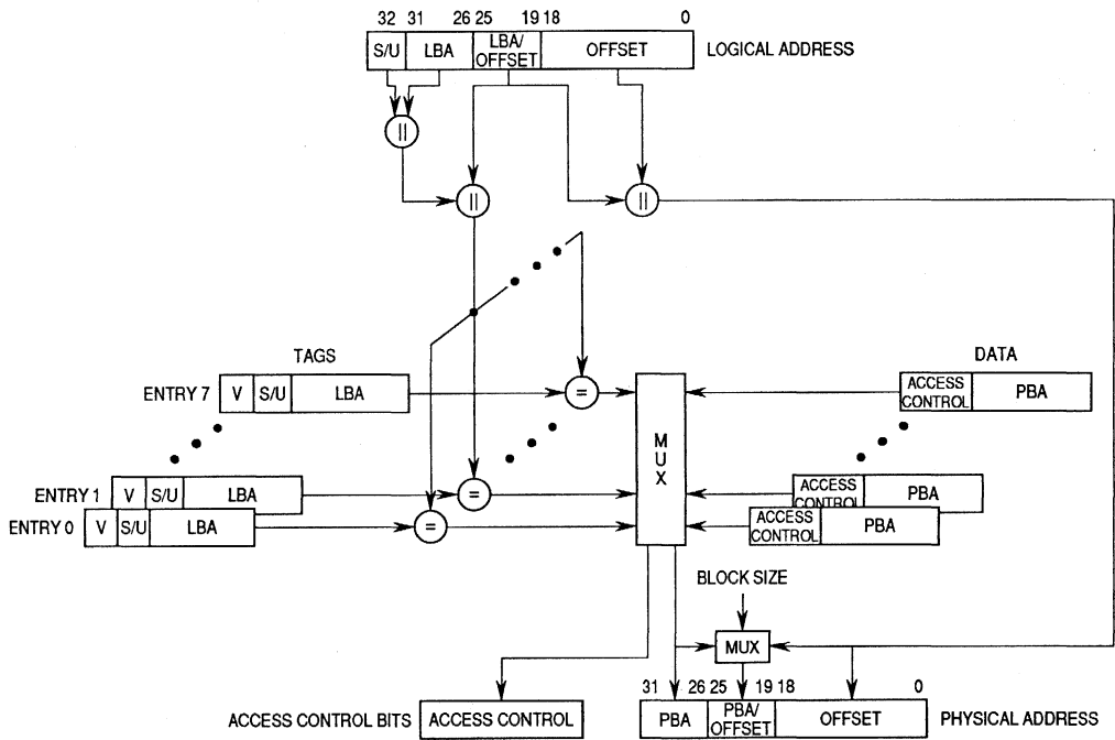
Figure 8-5. BATC Organization
