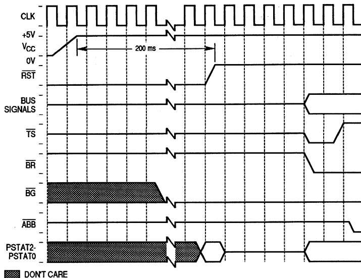
Figure 11-56. Initial Power-On Reset Timing
